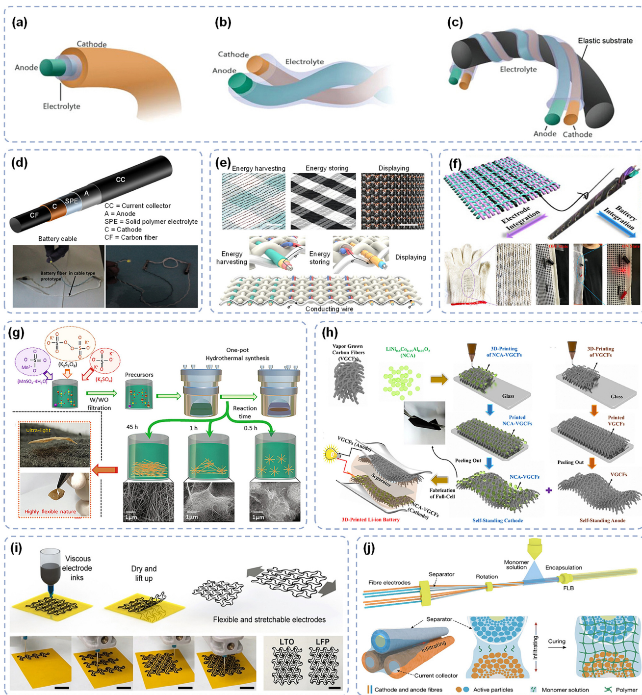
Fig. 3. (Color online) Progress of flexible LIBs. Schematic illustration of (a) coaxial, (b) twisted, and (c) stretchable 1D LIBs. Reprinted with permission from Ref. [9], Copyright © 2020, Wiley. (d) Schematic of battery cable and lighting of green light-emitting diode (LED) bulb (dim) in different bending conditions. Reprinted with permission from Ref. [22], Copyright © 2019, American Chemical Society. (e) Photographs of energy-harvesting (textile solar cells), energy-storage (textile batteries), and display textile modules for the all-textile integrated system. Reprinted with permission from Ref. [4], Copyright © 2022, Springer Nature. (f) Schematics to illustrate the easy integration of individual electrode fibers and batteries into commercial fabrics, and image that demonstrate the weavability of the printed electrode fiber into a woolen glove and the complete integration of a full battery into textile fabrics. Reprinted with permission from Ref. [33], Copyright © 2021, Elsevier. (g) Schematics for the one-pot hydrothermal synthesis, and features of freestanding films. Reprinted with permission from Ref. [40], Copyright © 2022, Elsevier. (h) Schematics of the 3D-printing process of self-standing electrodes. Reprinted with permission from Ref. [44], Copyright © 2022, Elsevier. (i) Suitably patterned stretchable electrodes fabricated by 3D printing. Reprinted with permission from Ref. [45], Copyright © 2020, Elsevier. (j) Fabrication of the fiber LIB with polymer gel electrolyte inspired by Boston ivy. Reprinted with permission from Ref. [8], Copyright © 2024, Springer Nature.
