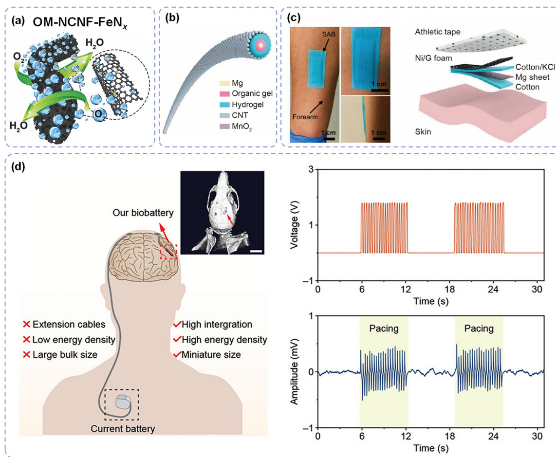
Fig. 9. (Color online) Configurations and applications of flexible MABs. (a) Schematic illustration of the ORR progress for OM-NCNF-FeN x nanofiber catalysts. Reprinted with permission from Ref. [204], Copyright © 2018, Wiley. (b) Schematic illustration of the fiber MAB. Reprinted with permission from Ref. [208], Copyright © 2021, Wiley. (c) Optical images of the batteries mounted onto a human forearm, and the schematic illustration of the sweat-activated MAB. Reprinted with permission from Ref. [212], Copyright © 2022, Elsevier. (d) Future visions for electrical brain stimulation, a voltage-time curve of the pulse power supplied by the brain stimulator powered by an MAB, and EEG signals before and during the electrical stimulation. Reprinted with permission from Ref. [211], Copyright © 2023, Wiley.
