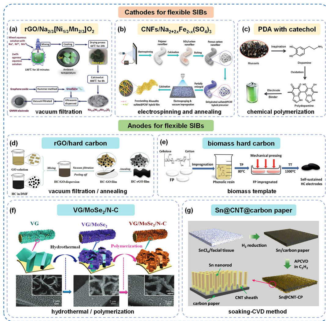
Fig. 4. (Color online) Flexible cathodes and anodes for SIBs. (a) Assembly process of rGO/Na 2/3 [Ni 1/3 Mn 2/3 ]O 2 free-standing composite. Reprinted with permission from Ref. [74], Copyright © 2014, The Royal Society of Chemistry. (b) Assembly process of CNFs/Na 2+2x Fe 2-x (SO 4 ) 3 . Reprinted with permission from Ref. [75], Copyright © 2016, The Royal Society of Chemistry. (c) Assembly process of PDA with catechol groups. Reprinted with permission from Ref. [79], Copyright © 2016, Wiley. (d) Assembly process of rGO/hard carbon. Reprinted with permission from Ref. [86], Copyright © 2018, Elsevier. (e) Assembly process, thermogravimetric analysis and cycling performance of biomass hard carbon. Reprinted with permission from Ref. [88], Copyright © 2020, The Royal Society of Chemistry. (f) Assembly process of VG/MoSe 2 /N-C. Reprinted with permission from Ref. [91], Copyright © 2017, Wiley. (g) Assembly process of Sn@CNT@carbon paper. Reprinted with permission from Ref. [84], Copyright © 2015, Elsevier.
