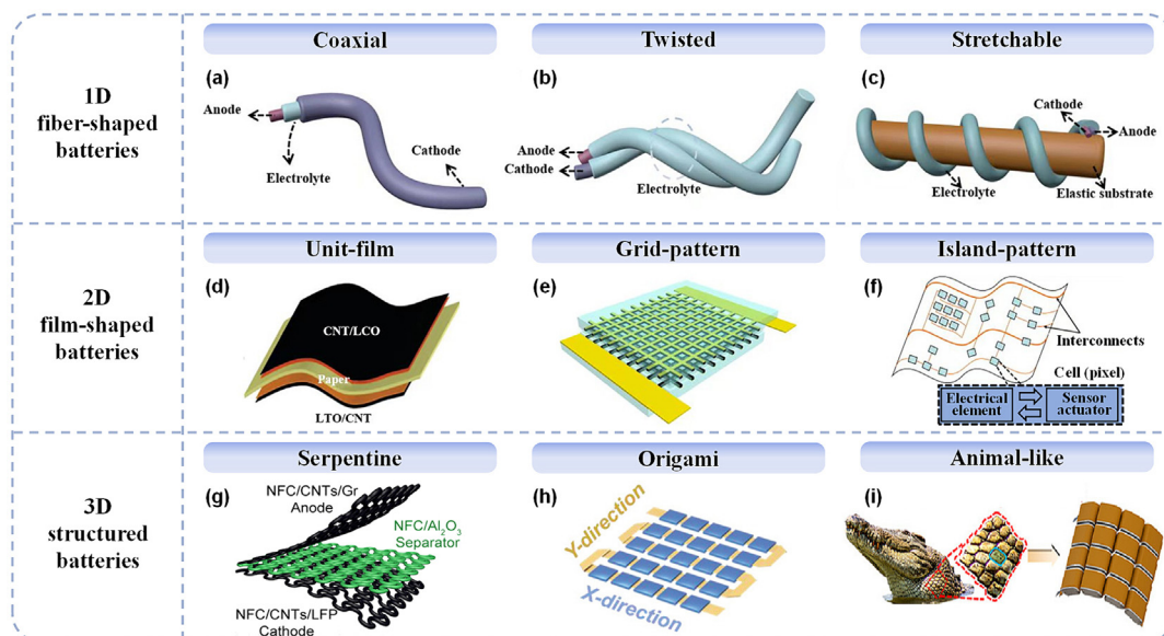
Fig. 2. (Color online) Typical structure of flexible batteries. (a) Coaxial structure; (b) twisted structure; (c) stretchable structure; (d) unit-film structure. Reprinted with permission from Ref. [14], Copyright © 2010, American Chemical Society. (e) Grid-pattern structure. Reprinted with permission from Ref. [15], Copyright © 2011, National Academy of Sciences. (f) Island-pattern structure. Reprinted with permission from Ref. [16], Copyright © 2004, Elsevier. (g) Serpentine structure. Reprinted with permission from Ref. [17], Copyright © 2022, Elsevier. (h) Origami structure. Reprinted with permission from Ref. [18], Copyright © 2021, Wiley. (i) Animal-like structure. Reprinted with permission from Ref. [19], Copyright © 2022, Elsevier.
