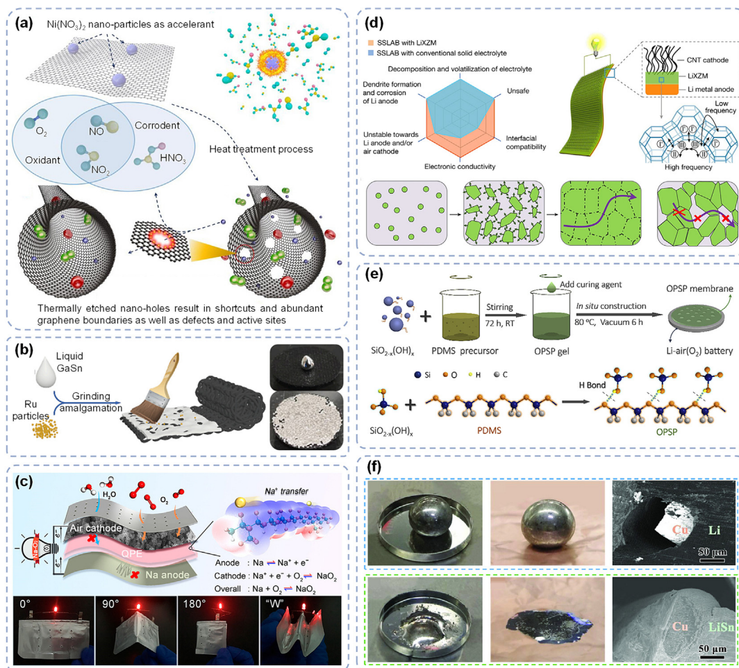
Fig. 7. (Color online) Design of flexible air cathodes, electrolytes, and metal anodes for flexible LABs and SABs. (a) Schematic illustration of the formation mechanism of nano-holes into the graphene layers for HPGF. Reprinted with permission from Ref. [150], Copyright © 2022, Elsevier. (b) Scheme of the preparation process of Ru/LM cathode. Reprinted with permission from Ref. [154], Copyright © 2023, Elsevier. (c) Schematic diagram of a SAB with the structure of sodium foil anode/QPE/air cathode and digital pictures of the LED powered by the integrated flexible SABs at different states. Reprinted with permission from Ref. [157], Copyright © 2020, American Chemical Society. (d) Schematic of the zeolite solid electrolyte, the SSLAB integrated with C-LiXZM, and comparison between the in-situ zeolite membrane growth method and traditional preparation method for inorganic solid electrolytes. Reprinted with permission from Ref. [159], Copyright © 2021, Springer Nature. (e) Schematic illustration of the main fabrication processes of OPSP and the hydrogen-bond interaction. Reprinted with permission from Ref. [162], Copyright © 2020, Elsevier. (f) Liquefied pure lithium and Li-Sn hybrid on the stainless steel and copper, and the cross-sectional SEM images of copper fiber coated with pure lithium and Li-Sn hybrid. Reprinted with permission from Ref. [163], Copyright © 2020, Wiley.
