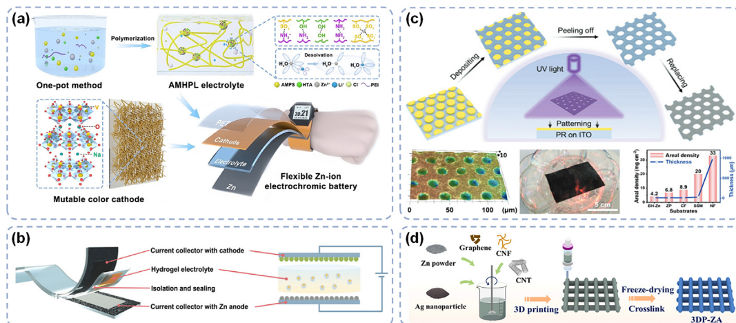
Fig. 6. (Color online) 2D flexible ZIBs. (a) Illustration of preparing the AMHPL electrolyte and \text{VO}_{\text{Na}^+} cathode for flexible electrochromic ZIBs assembly and application. Reprinted with permission from Ref. [122], Copyright © 2024, Wiley. (b) Schematic illustration of the flexible solid \text{Zn}||\text{Cu}_x\text{V}_2\text{O}_5 \cdot n\text{H}_2\text{O} batteries. Reprinted with permission from Ref. [113], Copyright © 2023, Wiley. (c) Fabrication and characterizations of BH-Zn electrode. Reprinted with permission from Ref. [126], Copyright © 2023, Wiley. (d) The schematic illustration of the preparation process of the 3D printing zinc anode and the electrochemical performances of the assembled full cells. Reprinted with permission from Ref. [127], Copyright © 2023, Elsevier.
