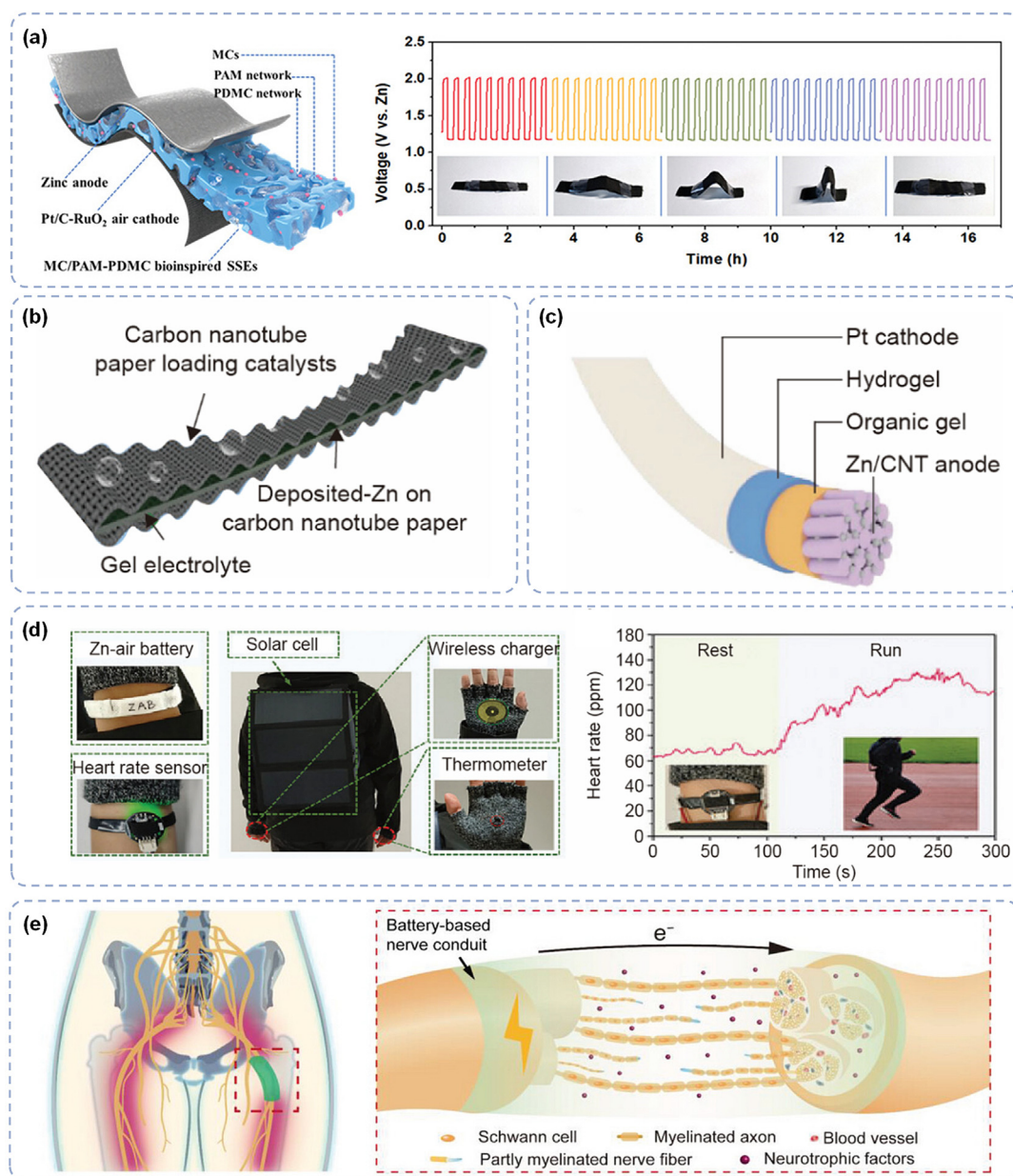
Fig. 8. (Color online) Configurations and applications of flexible ZABs. (a) Schematic illustration of flexible ZAB with a sandwich structure, and the galvanostatic discharge–charge curves under various mechanical deformations. Reprinted with permission from Ref. [182], Copyright © 2022, Wiley. (b) Schematic illustration of 800% stretchable planar-shaped ZAB. Reprinted with permission from Ref. [184], Copyright © 2019, Wiley. (c) Schematic of the hybrid fiber anode-based ZAB. Reprinted with permission from Ref. [190], Copyright © 2023, Wiley. (d) Schematic depicting how ZABs along with solar cells and sensors were integrated into wearable textiles, and real-time heart rate acquired by a sensor during rest and running. Reprinted with permission from Ref. [195], Copyright © 2023, Wiley. (e) Schematic illustration of the effect of ZAB-based nerve conduit for nerve regeneration. Reprinted with permission from Ref. [198], Copyright © 2023, Wiley.
